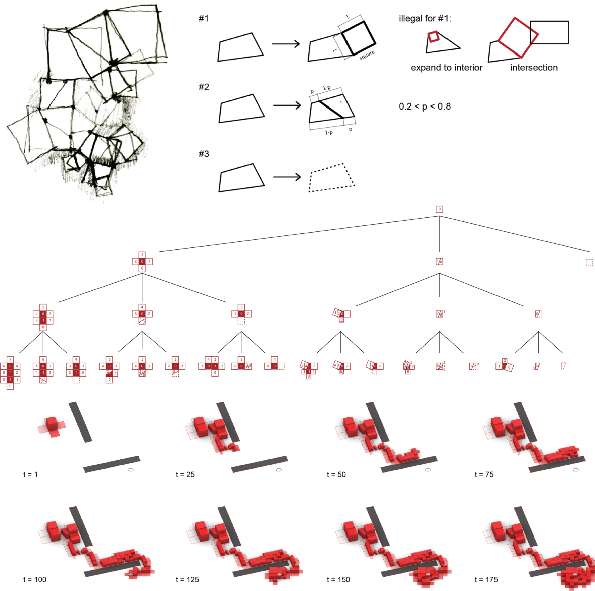
Figure 1. Constructive schema. Top , unstructured constructive schema of the qGrowth grammar; middle , qGrowth structured in a tree with a greedy best-first search algorithm that orders the frontier based on the Euclidean distance to a target; bottom , example of qGrowth generated by sampling. It follows the target behind a wall (ellipse).
